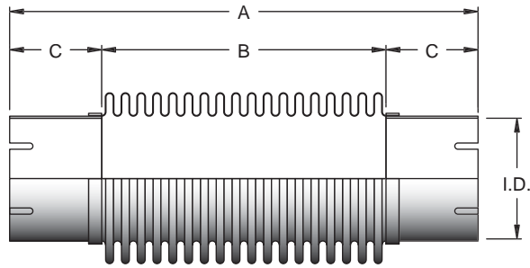
TUBE SIZE
